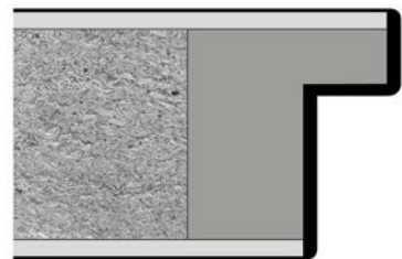
Invisible joint edgebands: homogeneous sealing of door panel edges
