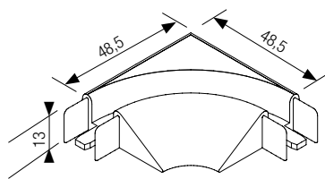
90°-Ecke TOP BASIC 8 mm
