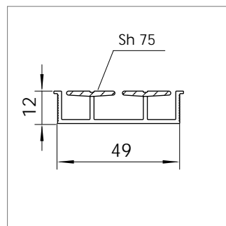
Mat.-Nr. 1611473 RAU-PVC 1309/7558
