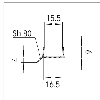
Mat.-Nr. 1610972 RAU-PVC 1107/8005
