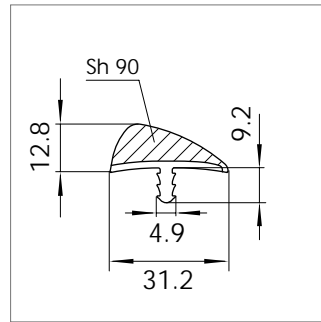
Mat.-Nr. 1712264* RAU-PVC 9708/9008
