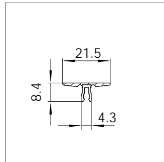
Mat.-Nr. 1628812 RAU-PVC 1309/7558
