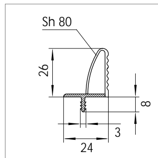
Mat.Nr. 1612503 RAU-PVC 1309/8000
