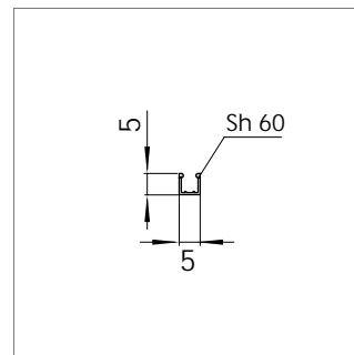
Mat.-Nr. 1628027/1628007 RAU-PVC 1107/6005
