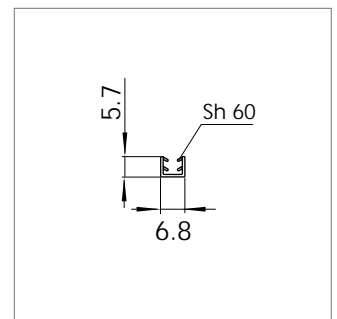
Mat.-Nr. 1625723 RAU-PVC 1309/8558
