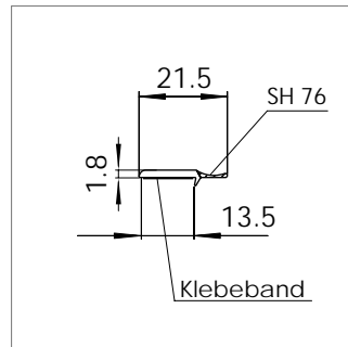
Mat.-Nr. 1618697 RAU-PVC 1107/7600
