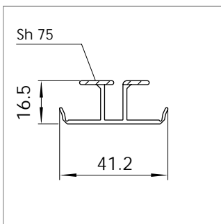
Mat.-Nr. 1618783 RAU-PVC 1309/7558
