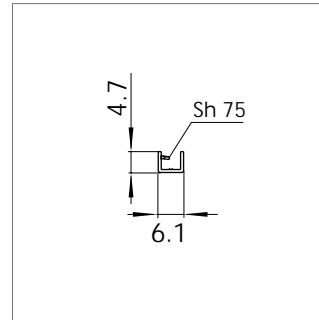
Mat.-Nr. 1626178 RAU-PVC 1107/6005
